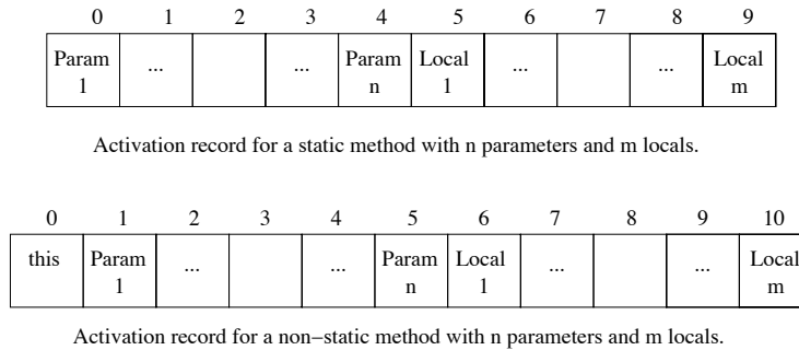
Figure 1: JVM Activation Records.
